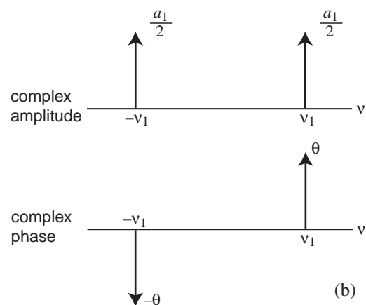
Fig. 1: Expressions of phases. (a) a_1 \cos 2\pi\nu_1 x . (b) a_1 \cos(2\pi\nu_1 x + \theta) .
