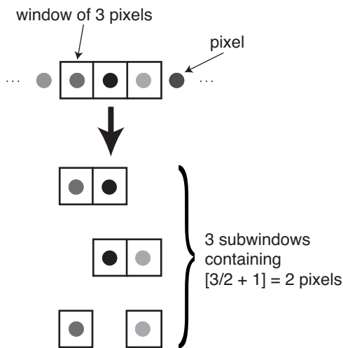
Fig. 1: Subwindows of \lceil n/2 + 1 \rceil pixels.
